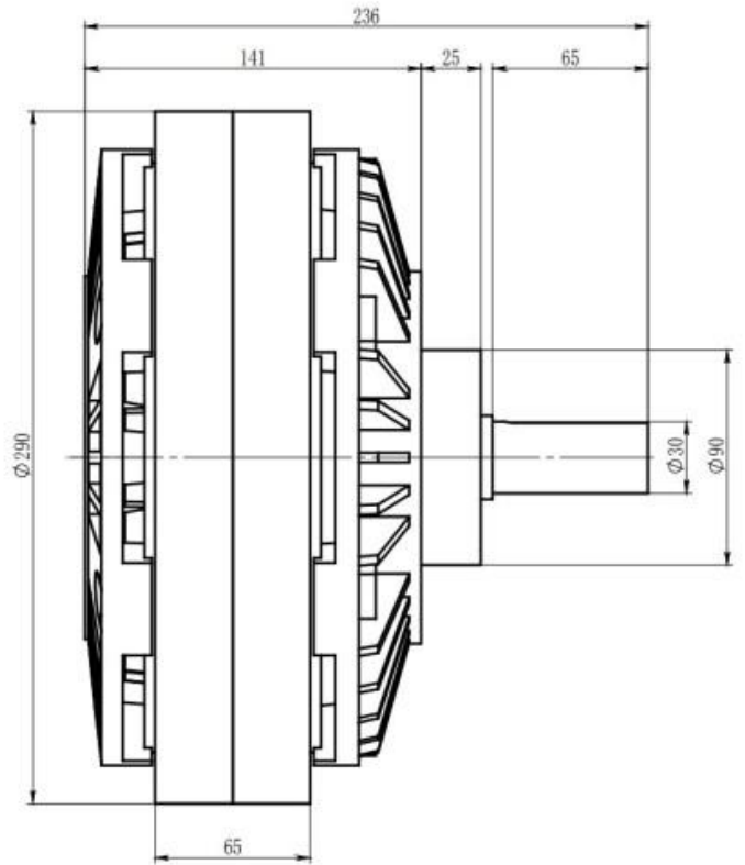
POWDER BRAKE SINGLE SHAFT 10 KG
